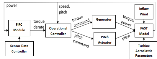
Fig.11 Simplified CART3 Model Block Diagram.
